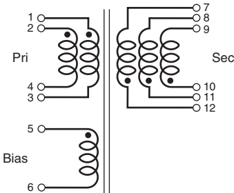
Primary windings and secondary windings to be connected in parallel on PCB board.
