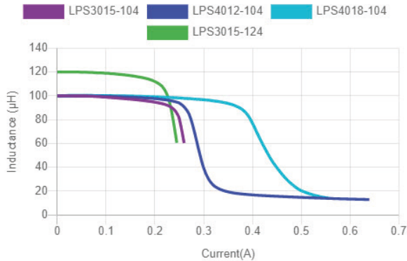
Figure 5. L vs. I curves at 25^{\circ}\text{C}
