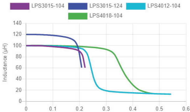
Figure 6. L vs. I curves derated for 85^{\circ}\text{C}
